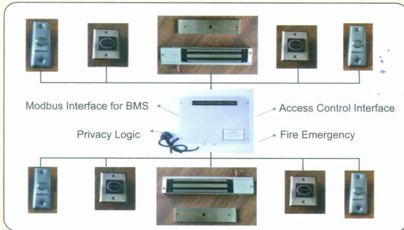
Typical 2 Door Interlocking System
